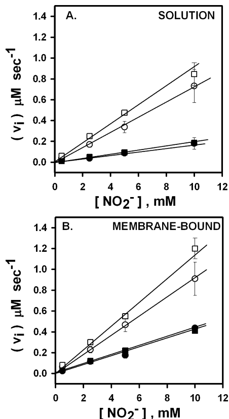
FIGURE 5: Plots of the initial velocity ( v_i ) vs [\text{NO}_2^-] for the reaction of \text{NO}_2^- with Hb(II). \text{NO}_2^- was reacted with preoxygenated or rapidly deoxygenated hemoglobin in solution (A) or bound to the cytoplasmic domain of band 3 (CDB3) (B). The results represented by the circles came from experimental determinations. Open circles were from rapid deoxygenation experiments, while closed circles were from preoxygenation experiments. The results represented by the squares were from model simulation studies. Open squares were from rapid deoxygenation simulations, while closed squares were from preoxygenation simulations. The experimental reactions were performed as described in the legend to Figure 4, and the initial velocities were calculated as described in the text. Quantitative values for the slopes of the lines in this figure are given in Table 1.
